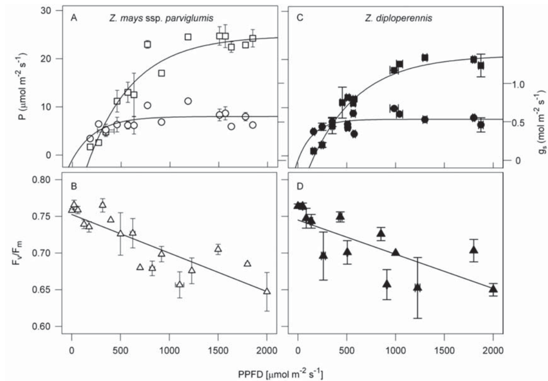
Figure 1. A,C: Net photosynthesis ( P ; squares) and stomatal conductance ( g_s ; circles); B,D: ratios of variable to maximum fluorescence ( F_v/F_m ) as a function of photosynthetic photon flux density (PPFD) in annual ( Z. mays ssp. parviglumis : A,B; open symbols) and perennial teosinte ( Z. diploperennis : C,D; closed symbols). Values are mean \pm standard error of measurements taken in 12 plants per species. Linear regressions for F_v/F_m as a function of irradiance were statistically significant at p \leq 0.01 in both species.
